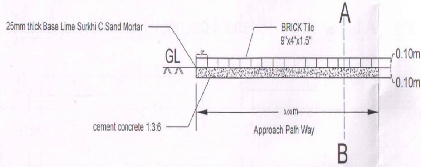
Sectional Elevation
